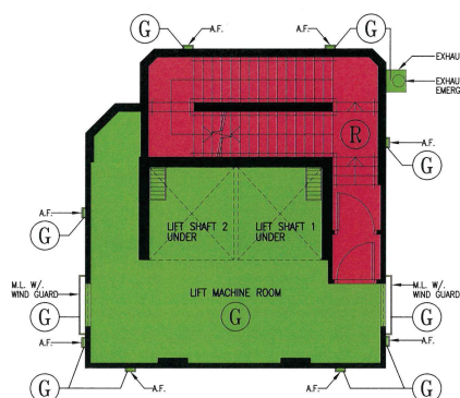
LIFT MACHINE ROOM FLOOR PLAN
