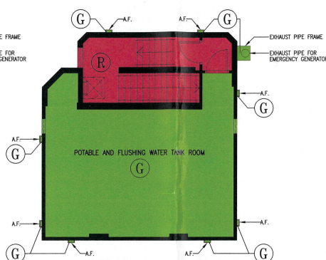
POTABLE AND FLUSHING WATER TANK ROOM FLOOR PLAN
