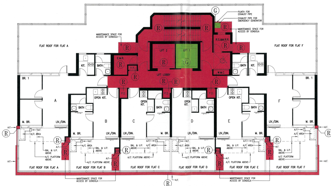
5TH FLOOR PLAN
